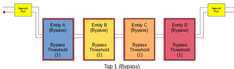
Figure 25 ATLB2 Chained Tap Mode (Bypass)
