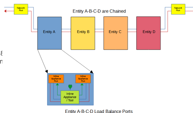
Figure 23 ATL2 Chained Tap Mode
