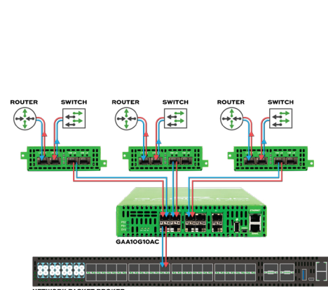
TAP Multiple Links & Aggregate to Packet Broker
