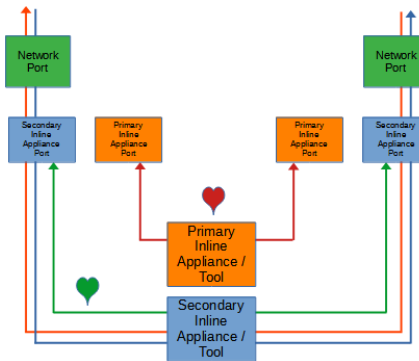
Figure 12 Primary-Secondary Tap Mode (Bypass)
