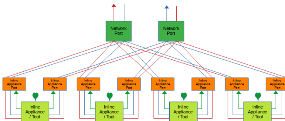
Figure 18 Load Balance Tap Mode (Inline)
