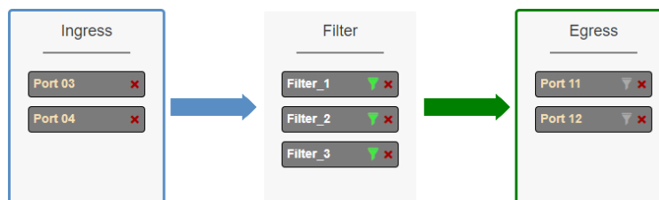
Figure 7 Egress Filter
