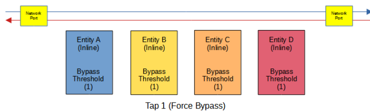
Figure 26 ATLB2 Chained Tap Mode (Force Bypass)
