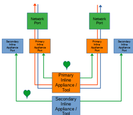
Figure 9 Primary-Secondary Tap Mode
