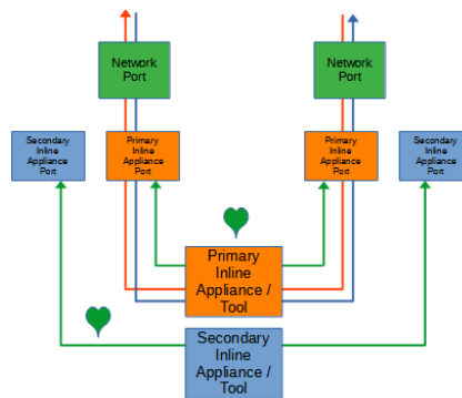
Figure 9 Primary-Secondary Tap Mode (Primary Inline)
