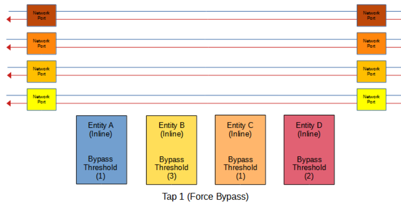
Figure 23 ATLB2 Chained Tap Mode (Force Bypass)
