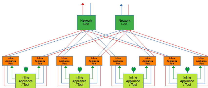
Figure 16 Load Balance Tap Mode (Inline)
