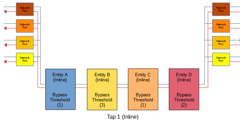
Figure 21 ATLB2 Chained Tap Mode (Inline)
