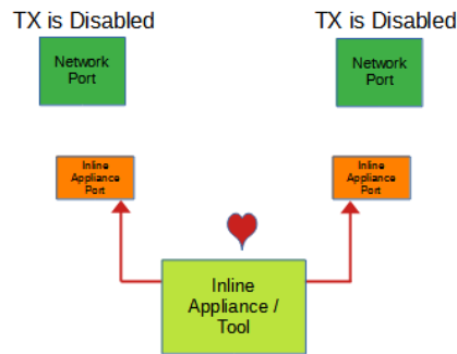
Figure 6 Default Tap Mode (Reverse Bypass)
