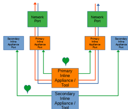
Figure 8 Primary-Secondary Tap Mode
