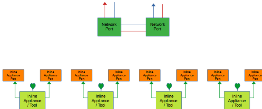
Figure 18 Load Balance Tap Mode (Force Bypass)
