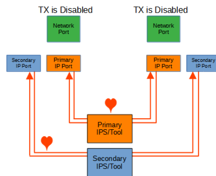
Figure 13 Primary-Secondary Tap Mode (Reverse Bypass)
