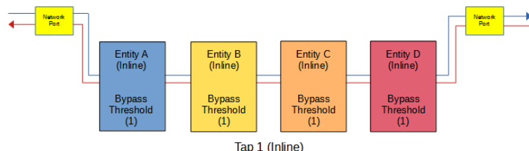
Figure 21 ATLB2 Chained Tap Mode (Inline)
