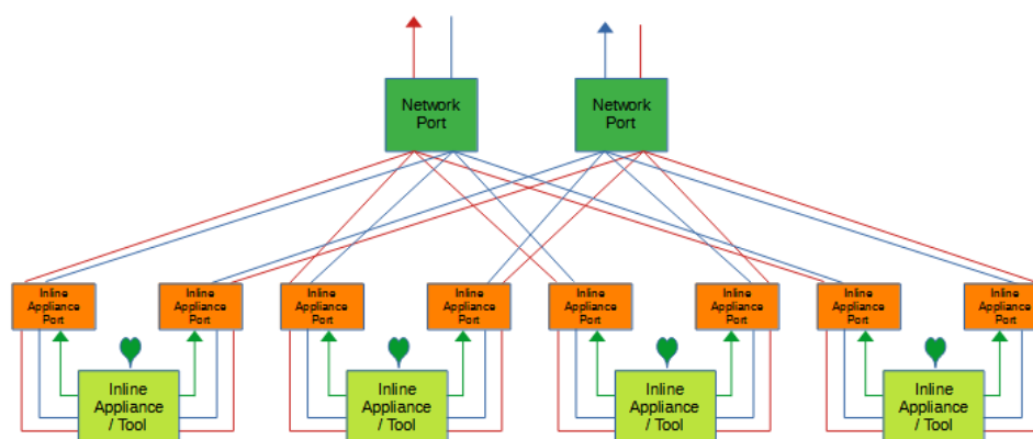
Figure 16 Load Balance Tap Mode (Inline)
