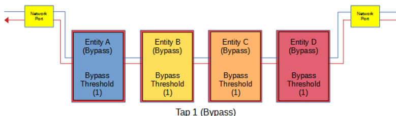
Figure 22 ATLB2 Chained Tap Mode (Bypass)
