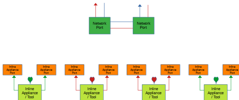
Figure 17 Load Balance Tap Mode (Bypass, Bypass Threshold=2)
