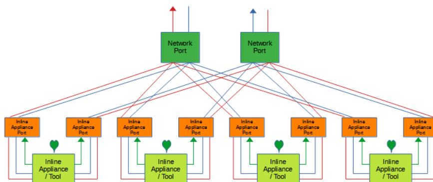
Figure 15 Load Balance Tap Mode
