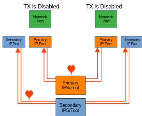
Figure 13 Primary-Secondary Tap Mode (Reverse Bypass)
