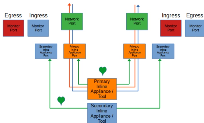
Figure 14 Primary-Secondary Tap Mode (Monitor Port)
