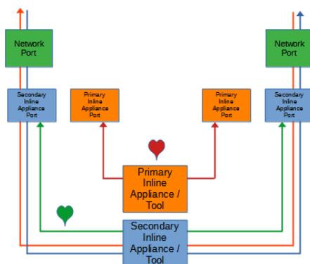
Figure 11 Primary-Secondary Tap Mode (Bypass)
