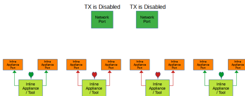
Figure 19 Load Balance Tap Mode (Reverse Bypass, Bypass Threshold=2)
