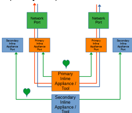
Figure 9 Primary-Secondary Tap Mode (Primary Inline)
