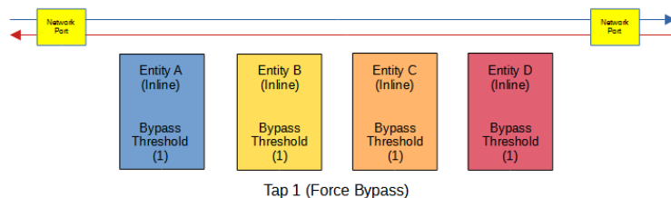
Figure 23 ATLB2 Chained Tap Mode (Force Bypass)
