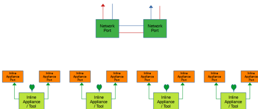
Figure 18 Load Balance Tap Mode (Force Bypass)
