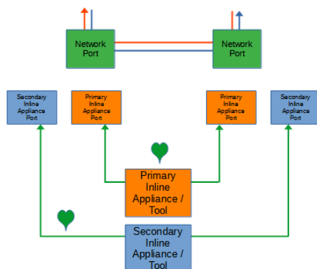
Figure 12 Primary-Secondary Tap Mode (Force Bypass)
