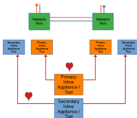
Figure 11 Primary-Secondary Tap Mode (Bypass)
