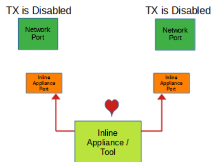
Figure 6 Default Tap Mode (Reverse Bypass)
