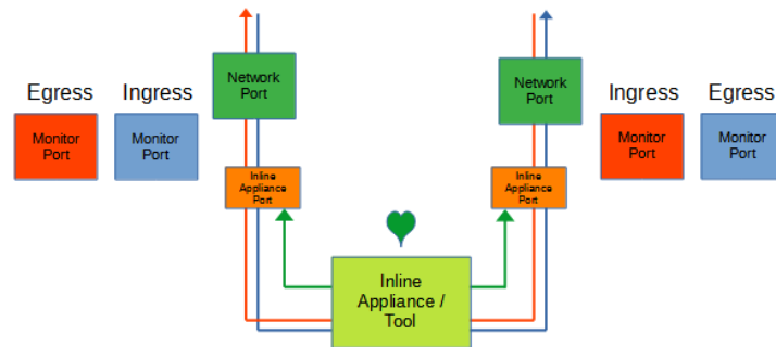
Figure 7 Default Tap Mode (Monitor Port)
