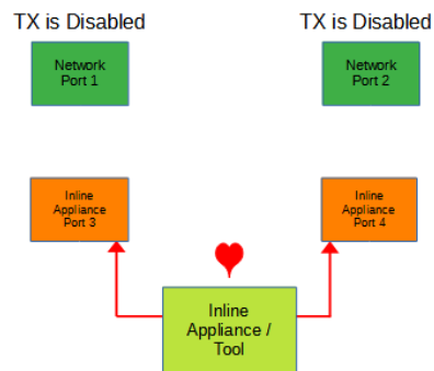
Figure 27 Bypass Filter Mode (Reverse Bypass)
