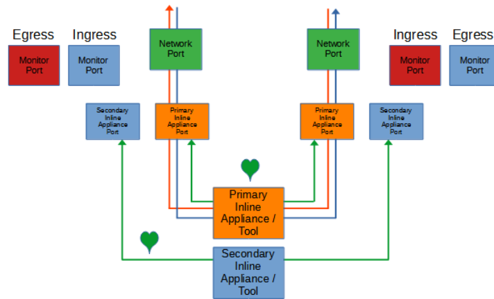
Figure 14 Primary-Secondary Tap Mode (Monitor Port)
