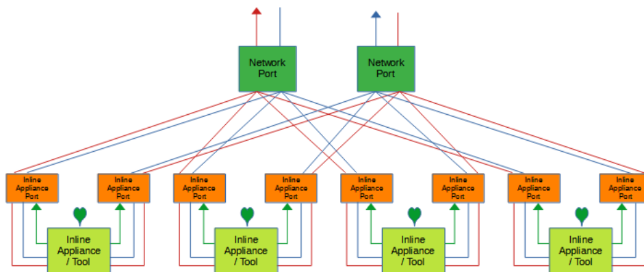
Figure 16 Load Balance Tap Mode (Inline)
